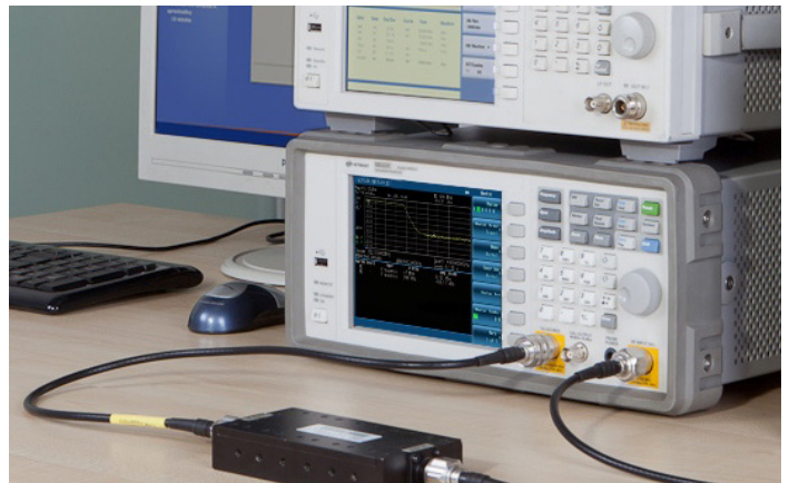
Figure 4. Transmission measurement setup
