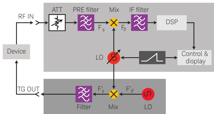
Figure 1. Block diagram of tracking generator
