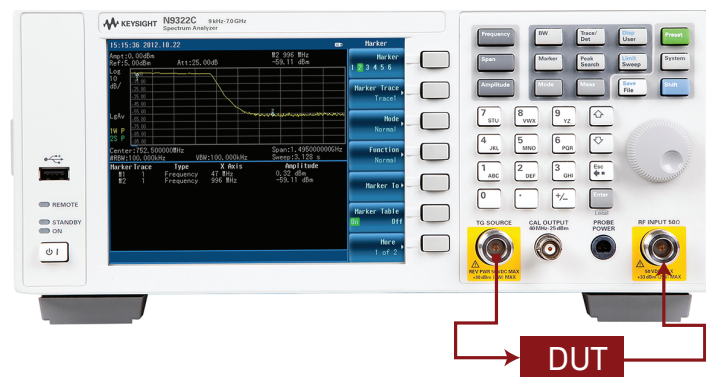
Figure 2. Using N9322C and its tracking generator for scalar network analysis
